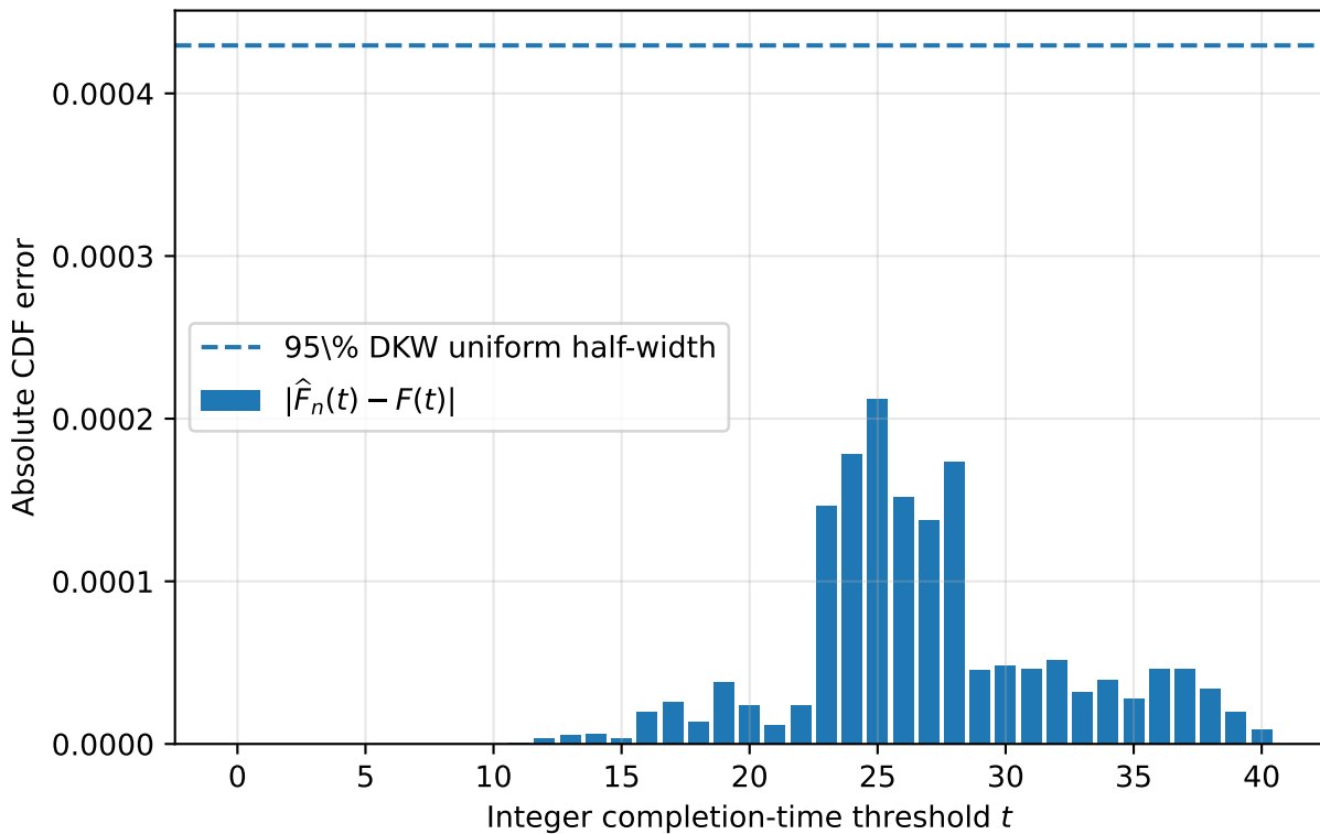
Absolute Monte Carlo CDF error
